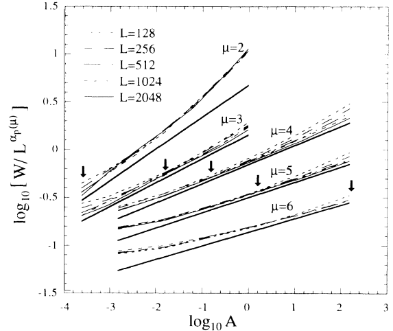
FIG. 3. Rescaled surface width W/L^{\alpha_p(\mu)} against noise intensity A on a log-log scale for \mu = 2 to 6. The vertical scale is shifted by 1.5, 0.8, 0.4, 0, and -0.4 , respectively. The arrows and the solid lines are explained in the text.
