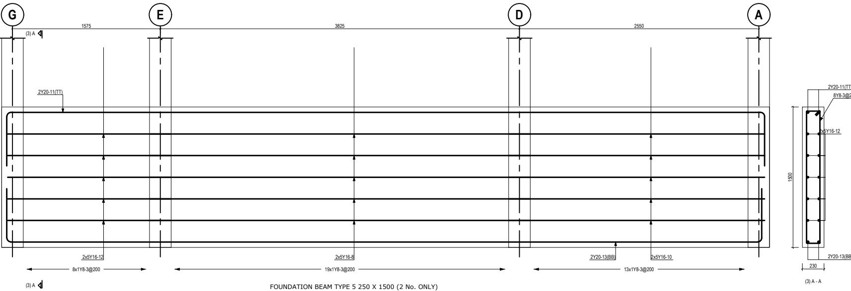
FOUNDATION BEAM TYPE 5 250 X 1500 (2 No. ONLY)
