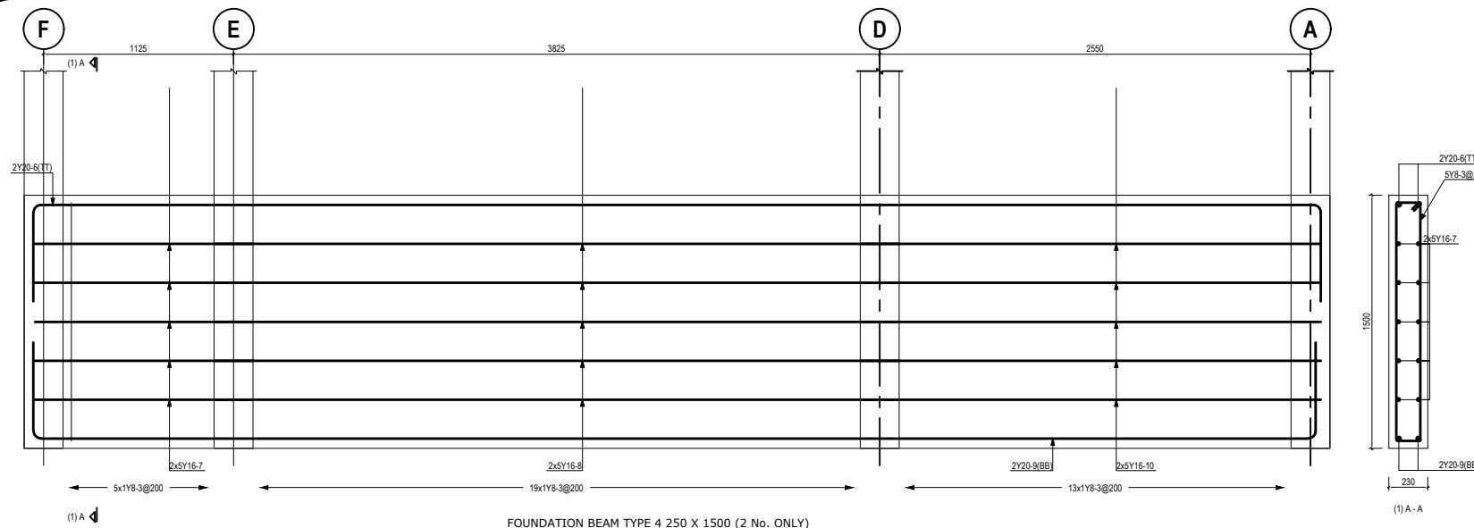
FOUNDATION BEAM TYPE 4 250 X 1500 (2 No. ONLY)
