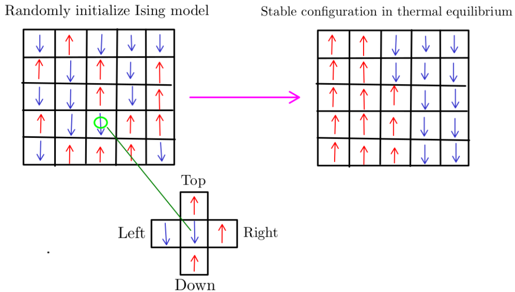
Figure 6.18: Metropolis algorithm illustration
