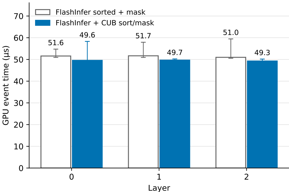
Complete exact top-k · Q1, k = 2,048
