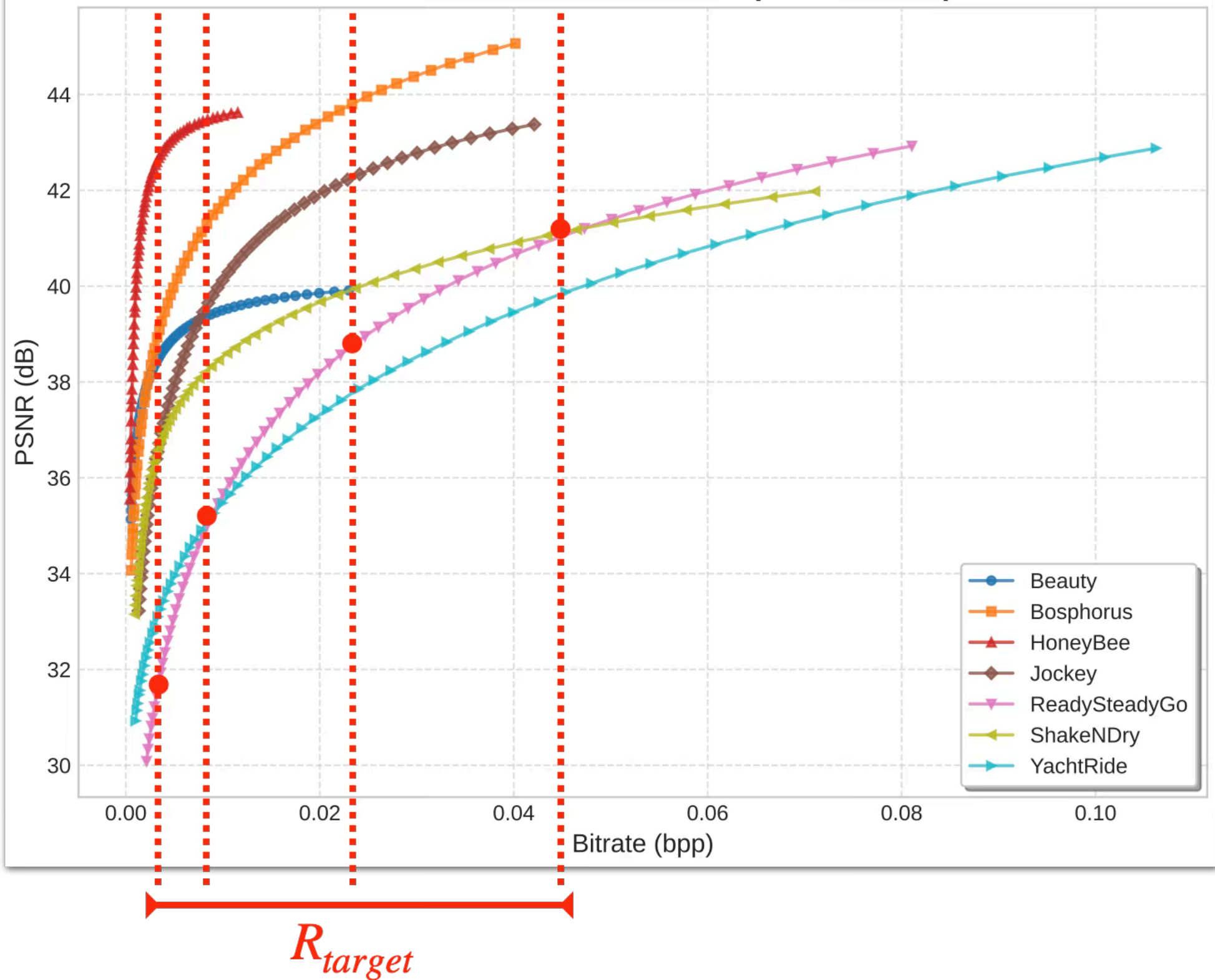
Rate-Distortion Performance (UVG Dataset)
