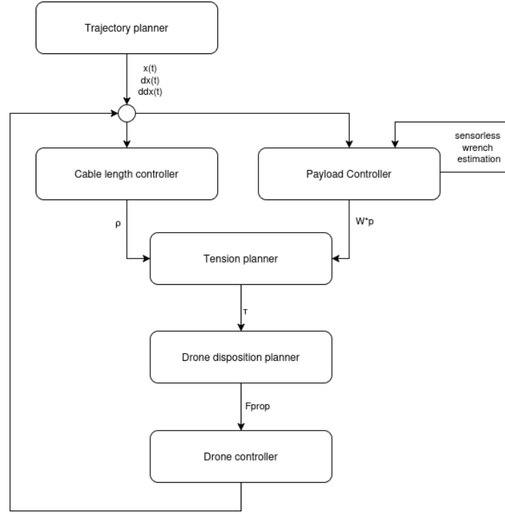
Figure 3.5: High level control scheme
