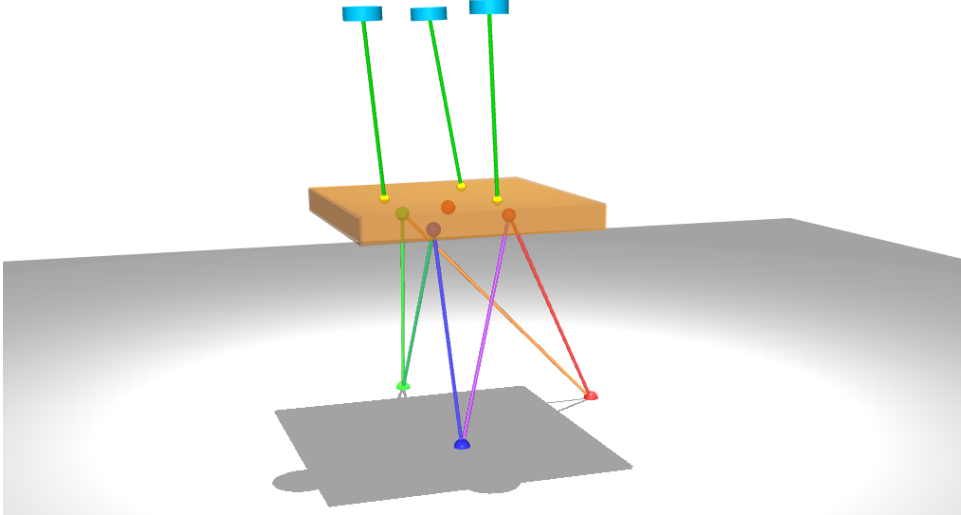
Figure 2.5: Over actuated ACTS with 6 ground cables and 3 UAVs
