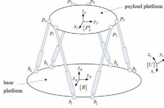
Figure 3.6: Gough Stewart schematics [2]
