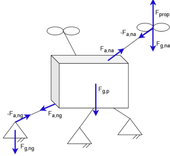
Figure 2.2: Forces acting on the ACTS
