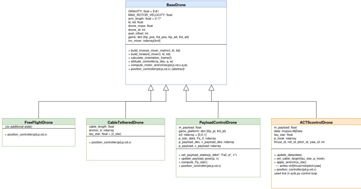
Figure 5.1: Class Diagram
