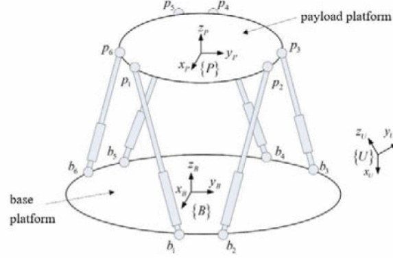
Figure 2.9: Gough Stewart schematics [?]
