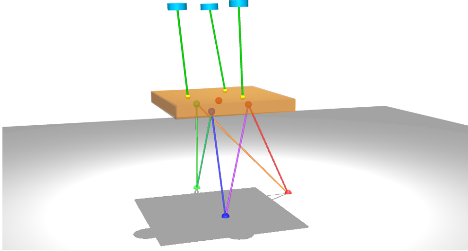
Figure 2.7: Over actuated ACTS with 6 ground cables and 3 UAVs
