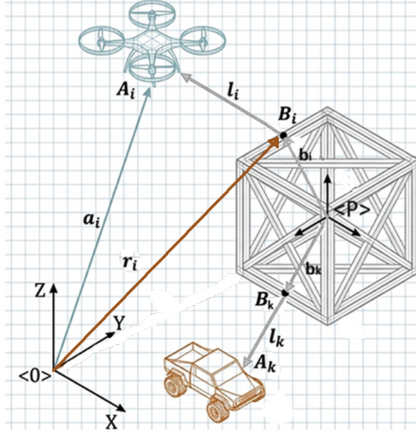
Figure 1.1: Graphical representation of the platform
