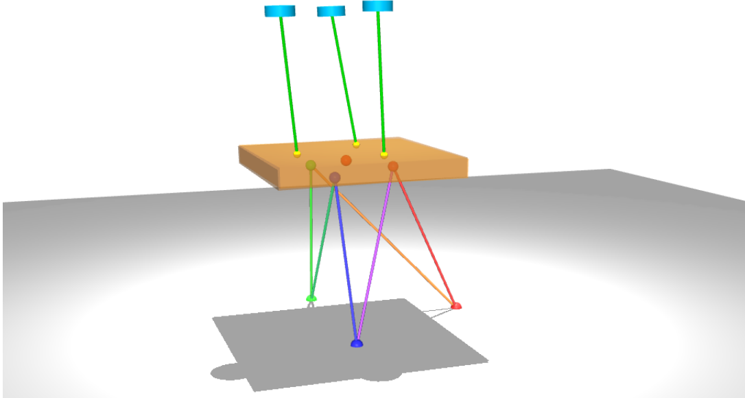
Figure 3.3: Over actuated ACTS with 6 ground cables and 3 UAVs
