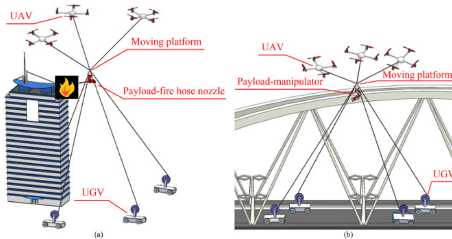
Figure 2.1: ACTRs with land-fixed winches for firefighting applications (a) and repair of a large bridge (b) [?]
