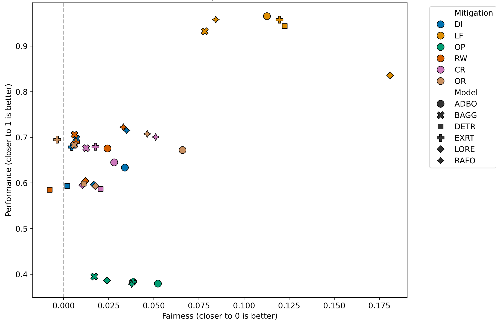
Fairness vs Performance Fairness: EOD | Performance: Pre
