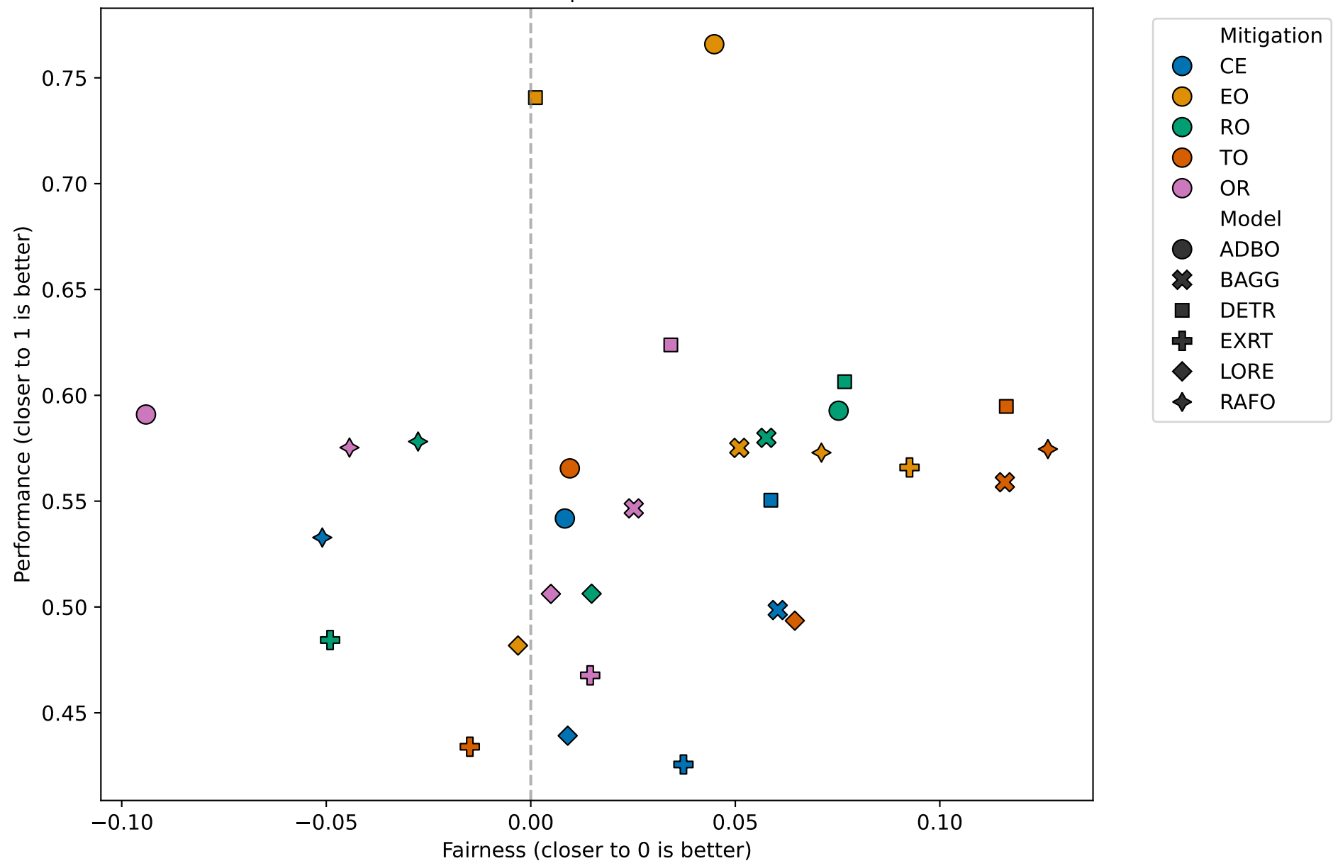
Fairness vs Performance Fairness: FNP | Performance: Rec
