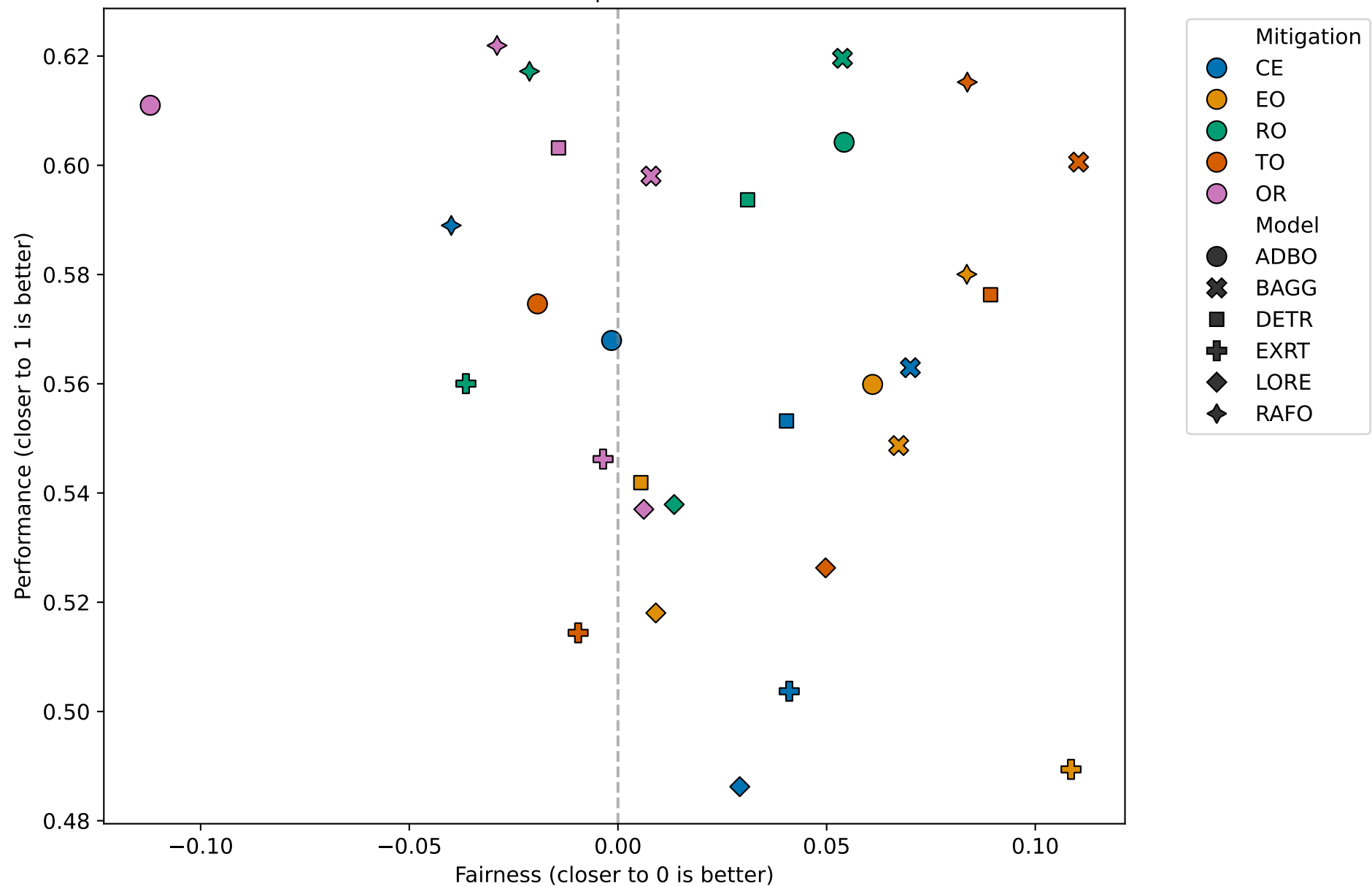
Fairness vs Performance Fairness: FOR | Performance: F1
