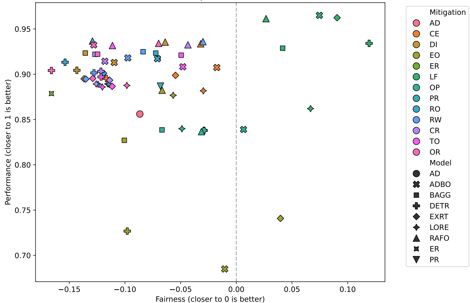
Fairness vs Performance Fairness: FPP | Performance: Acc
