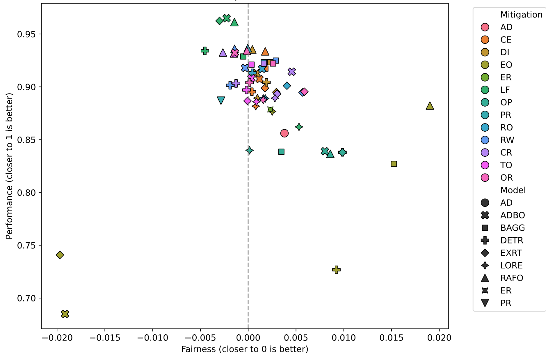
Fairness vs Performance Fairness: OAE | Performance: Acc
