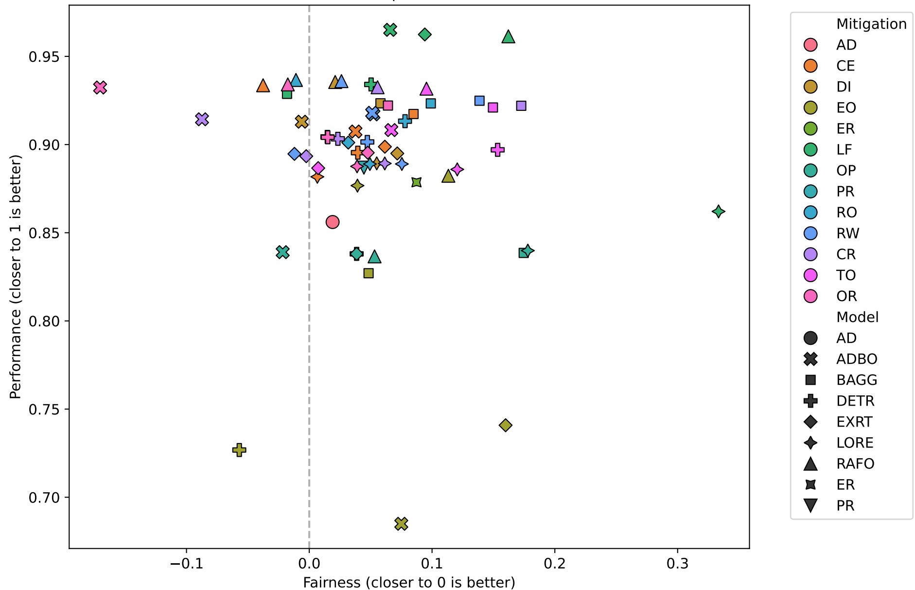
Fairness vs Performance Fairness: TEQ | Performance: Acc
