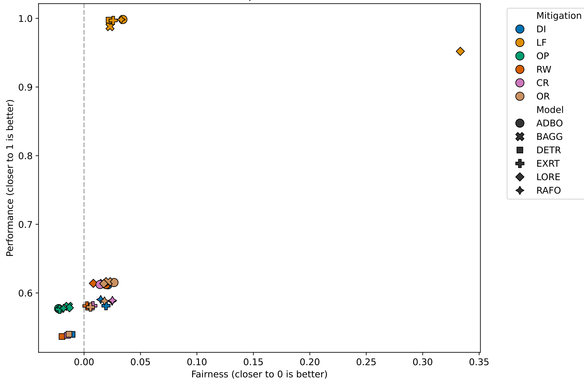
Fairness vs Performance Fairness: CUA | Performance: Acc
