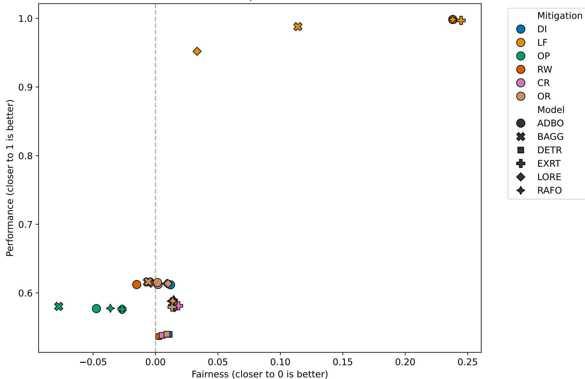
Fairness vs Performance Fairness: EOD | Performance: Acc
