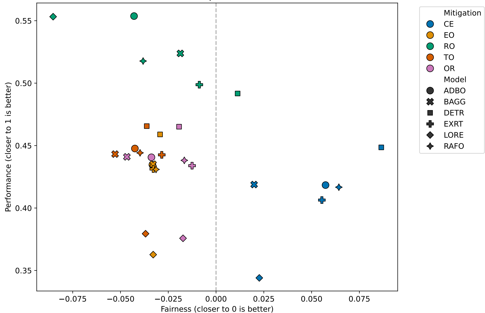
Fairness vs Performance Fairness: FPP | Performance: F1
