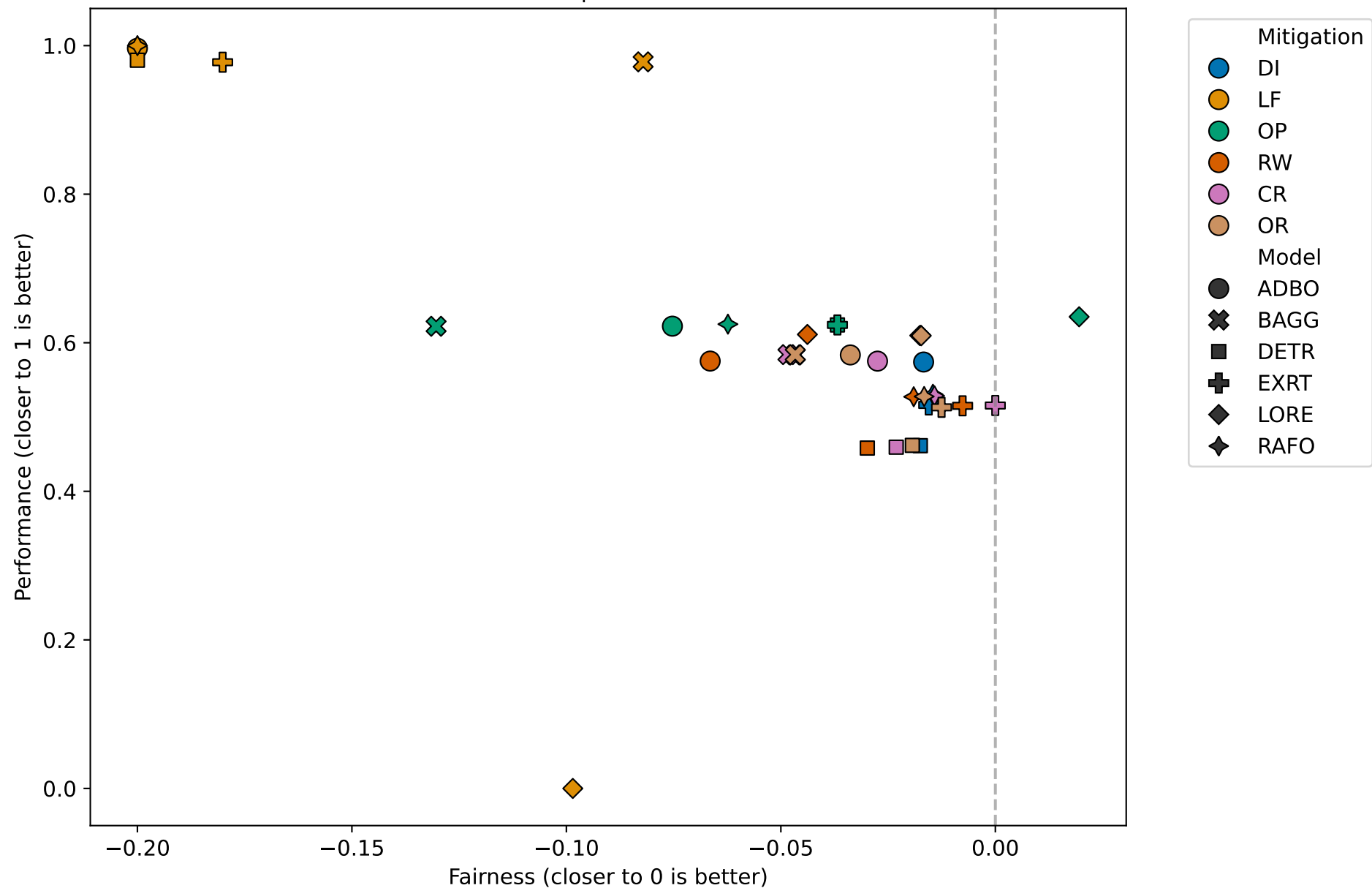
Fairness vs Performance Fairness: FPP | Performance: Pre
