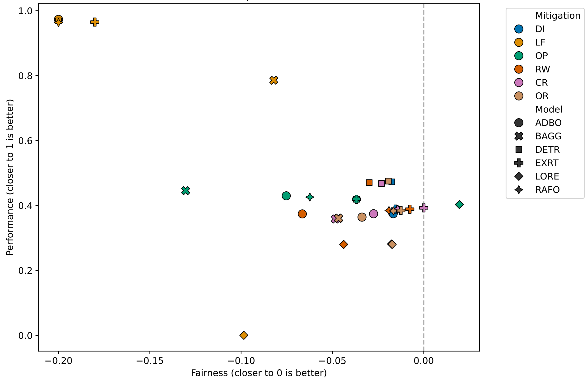
Fairness vs Performance Fairness: FPP | Performance: Rec
