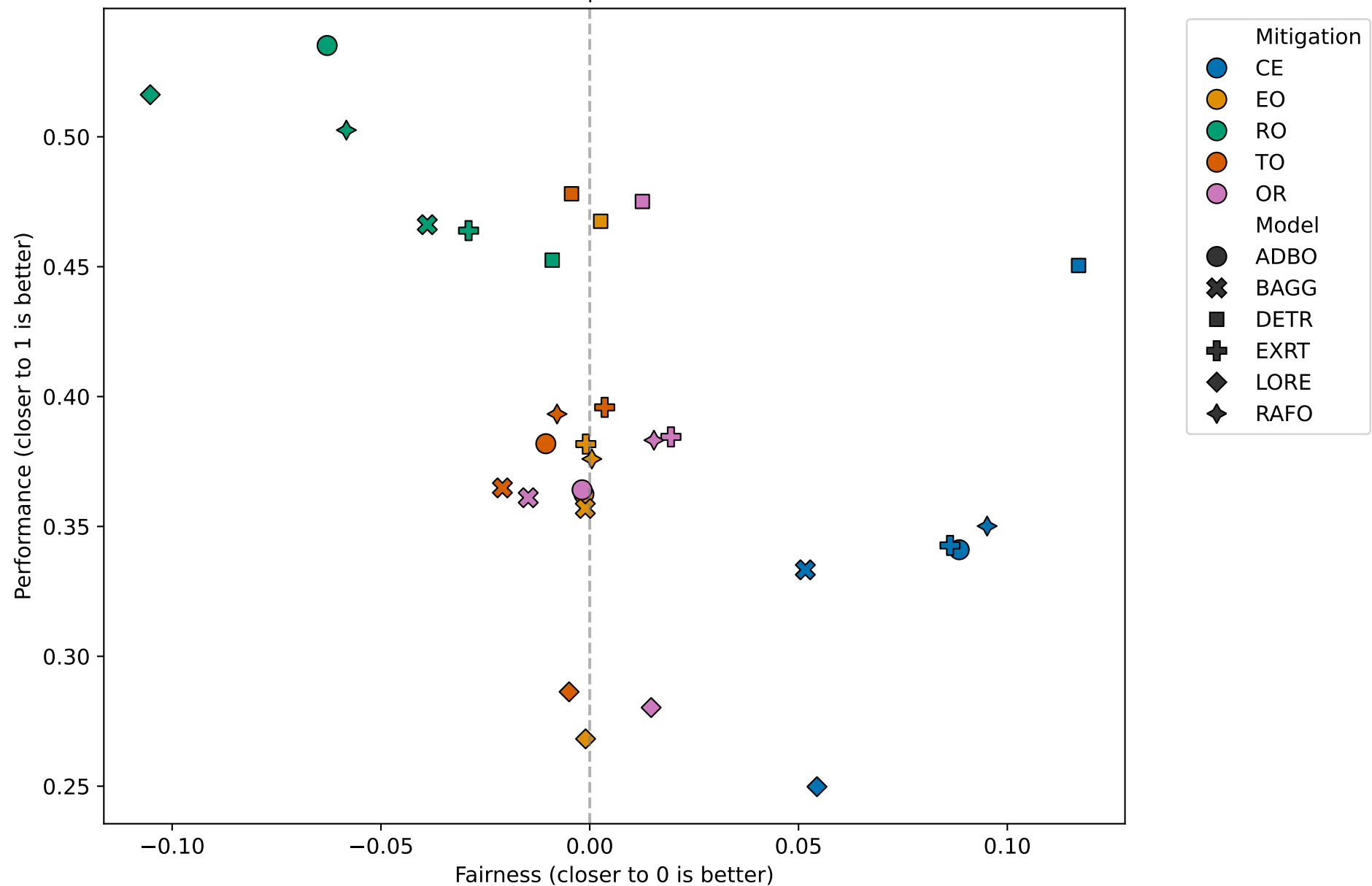
Fairness vs Performance Fairness: PEQ | Performance: Rec
