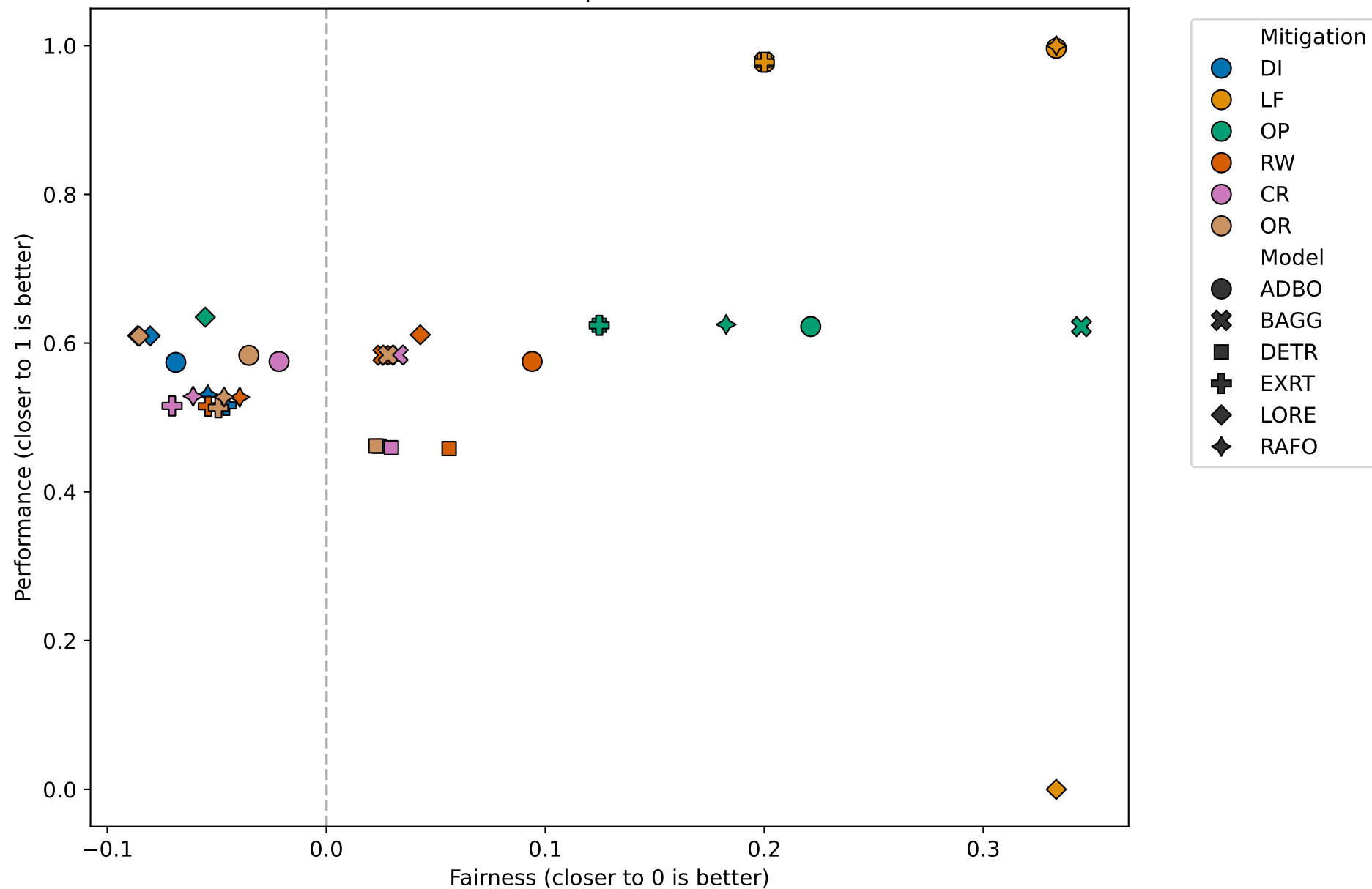
Fairness vs Performance Fairness: TEQ | Performance: Pre
