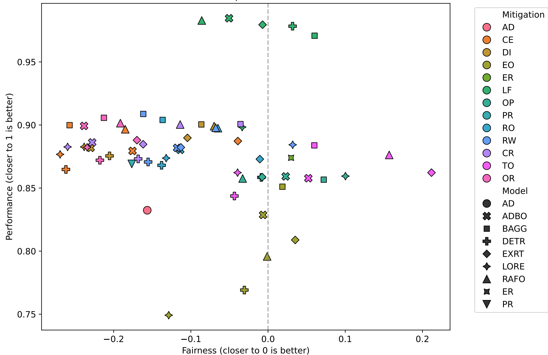
Fairness vs Performance Fairness: EOP | Performance: Acc
