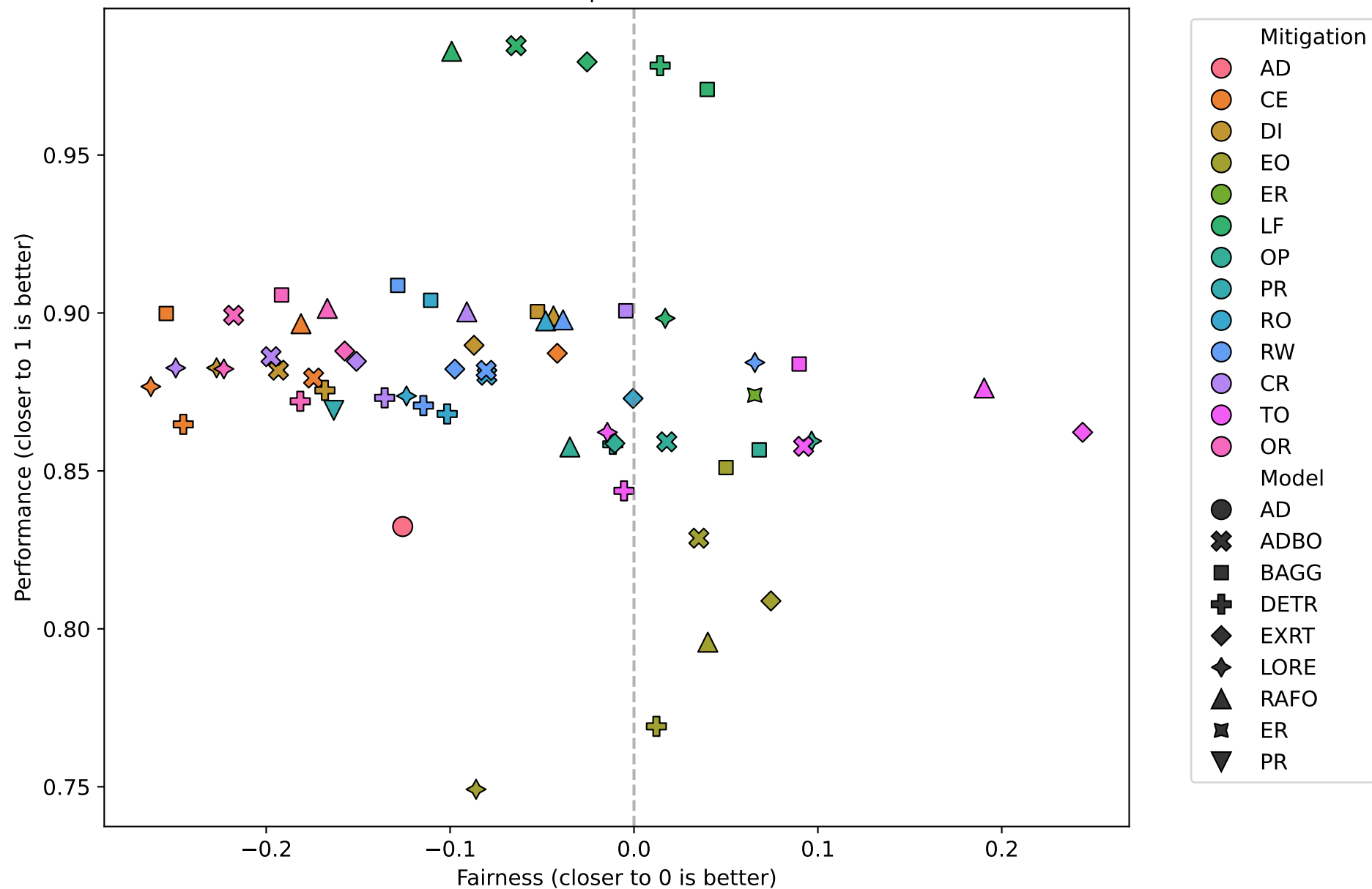
Fairness vs Performance Fairness: FNP | Performance: Acc
