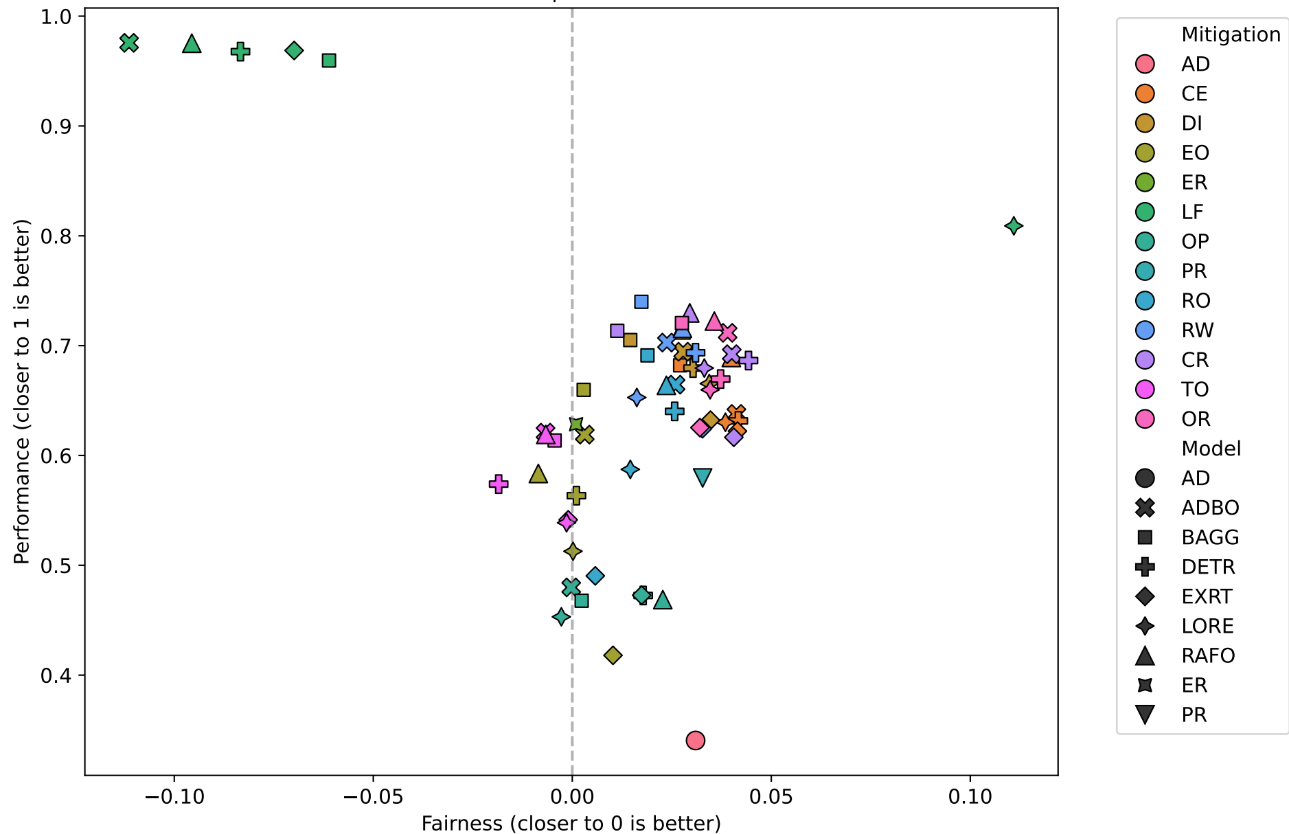
Fairness vs Performance Fairness: GFA | Performance: F1
