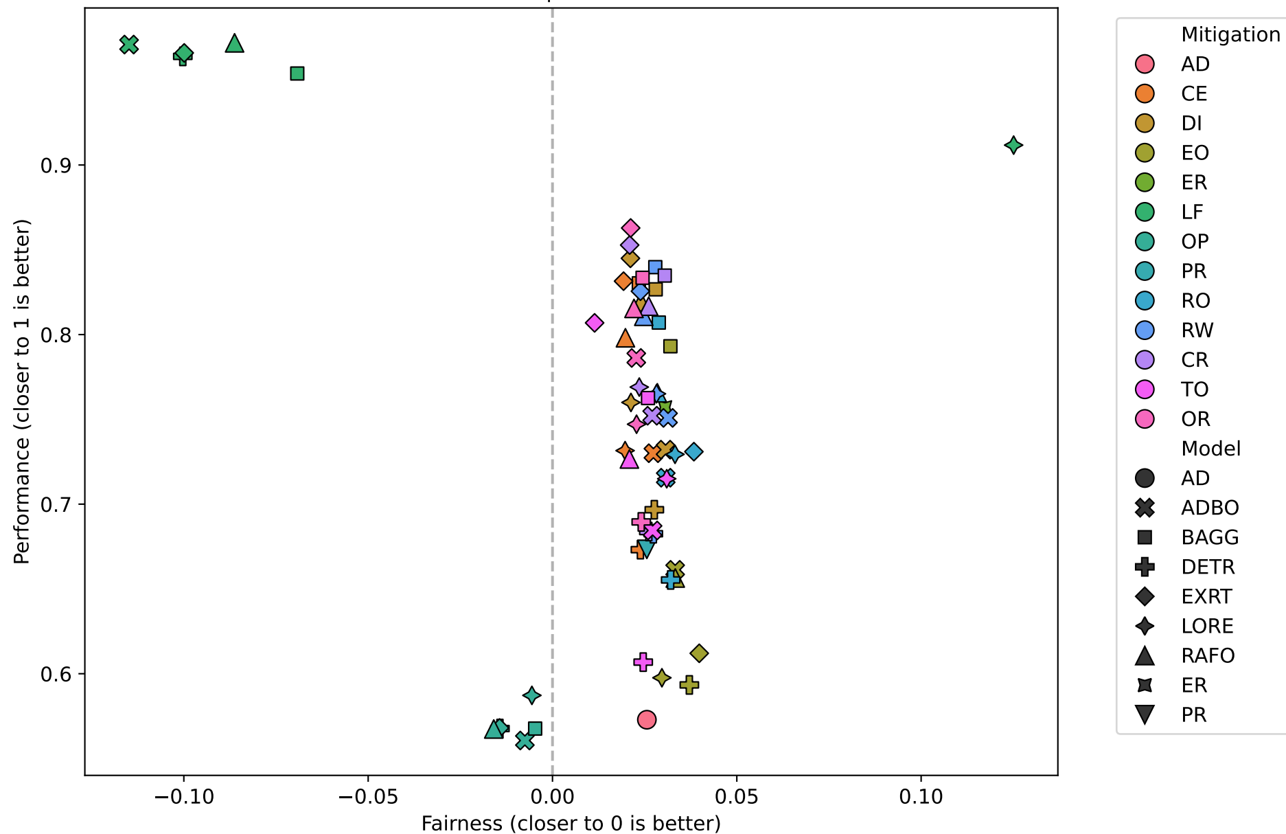
Fairness vs Performance Fairness: PPA | Performance: Pre
