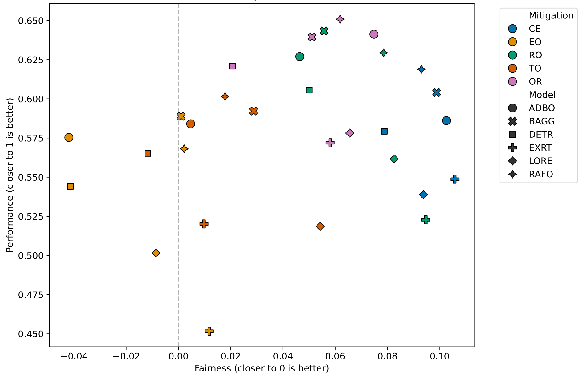
Fairness vs Performance Fairness: CUA | Performance: F1
