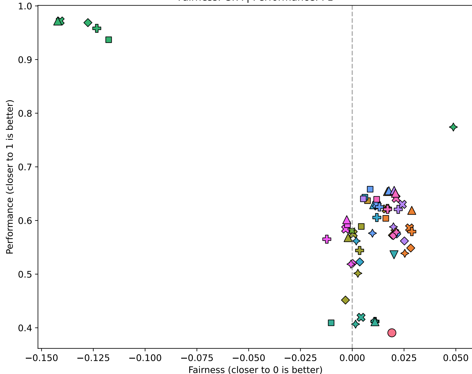
Fairness vs Performance Fairness: GFA | Performance: F1
