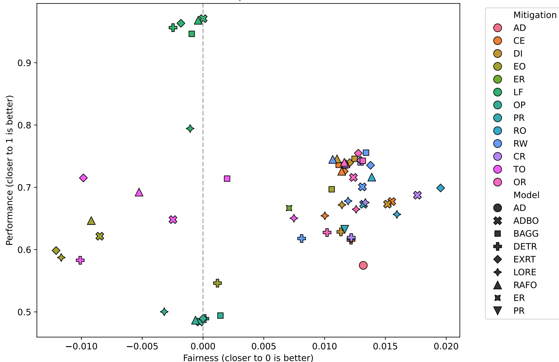
Fairness vs Performance Fairness: OAE | Performance: Pre
