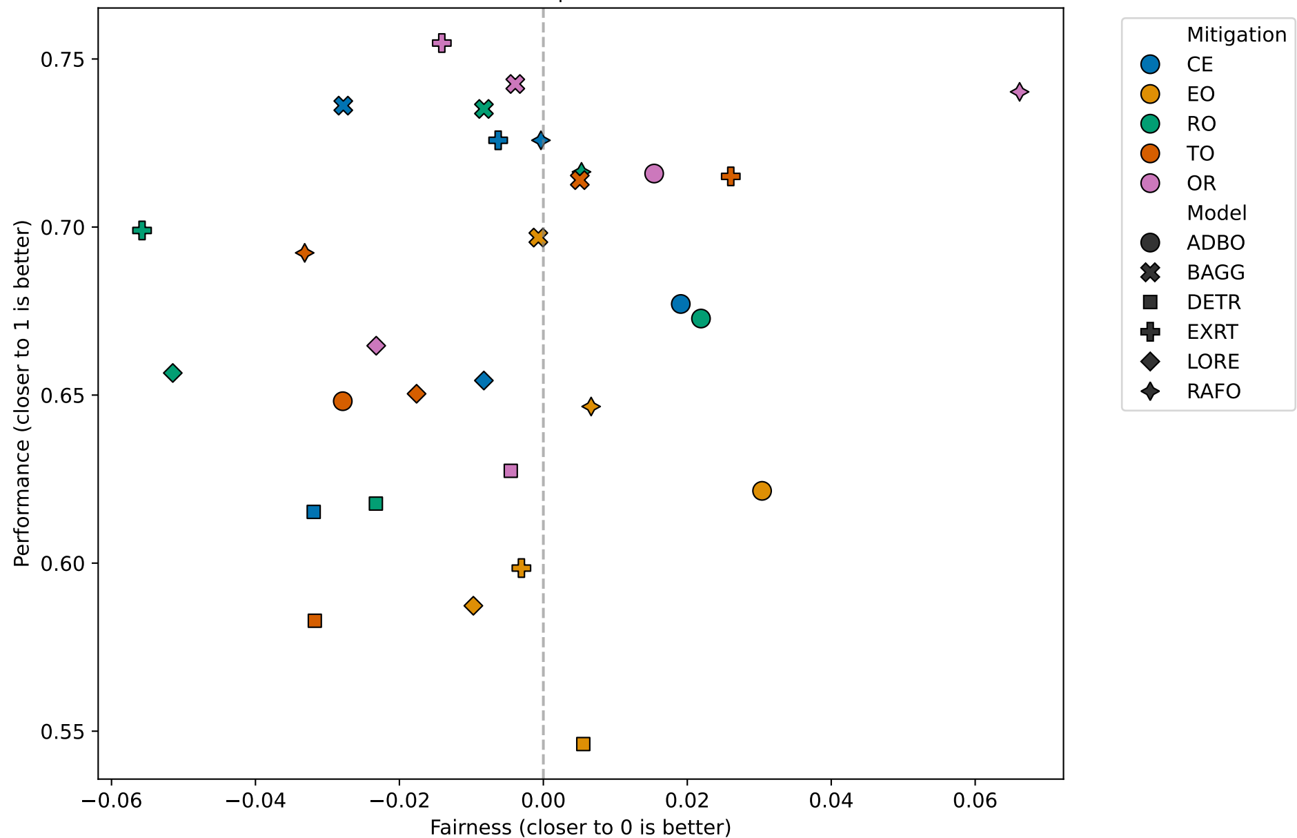
Fairness vs Performance Fairness: PEQ | Performance: Pre
