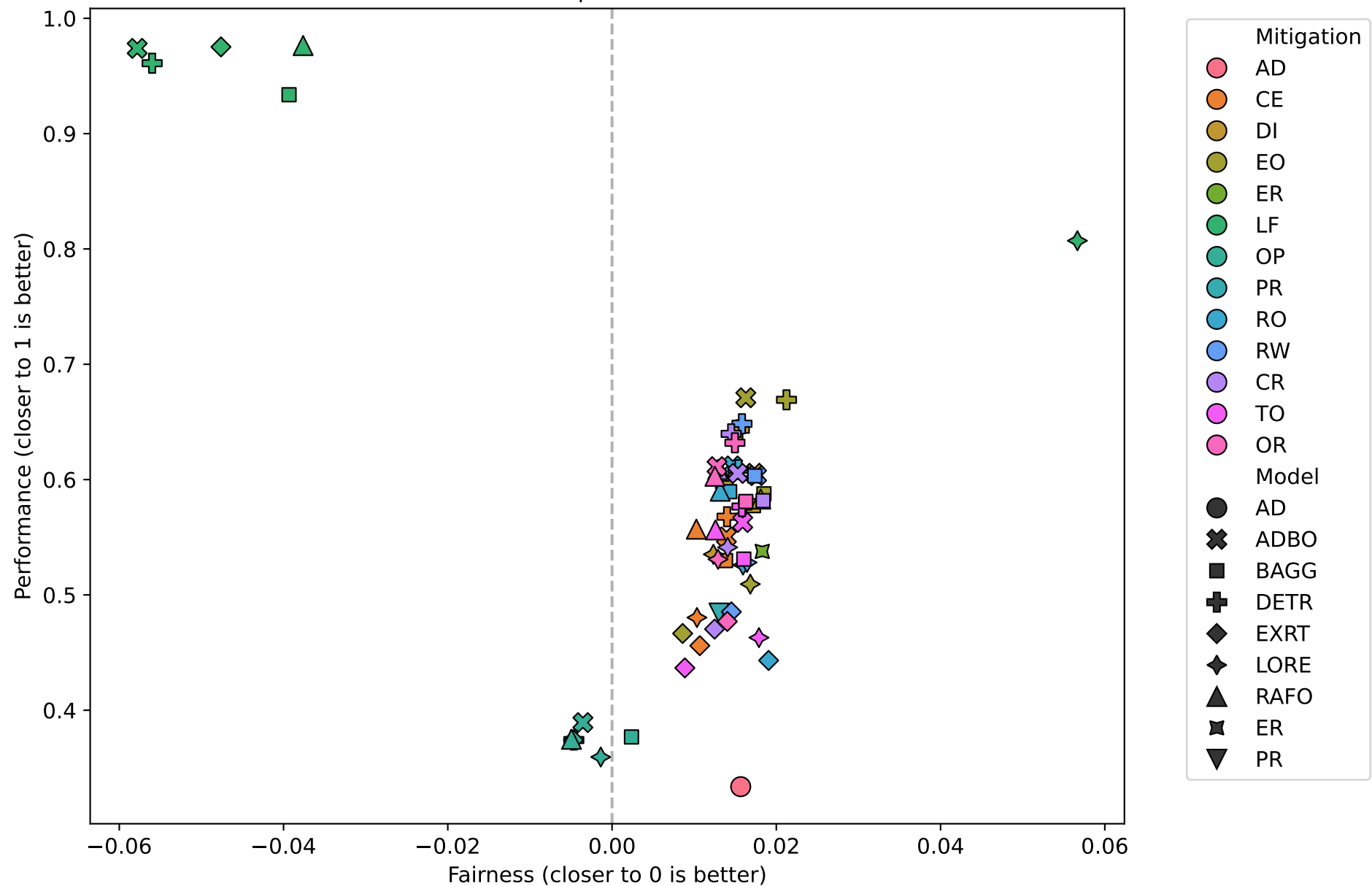
Fairness vs Performance Fairness: PPA | Performance: Rec
