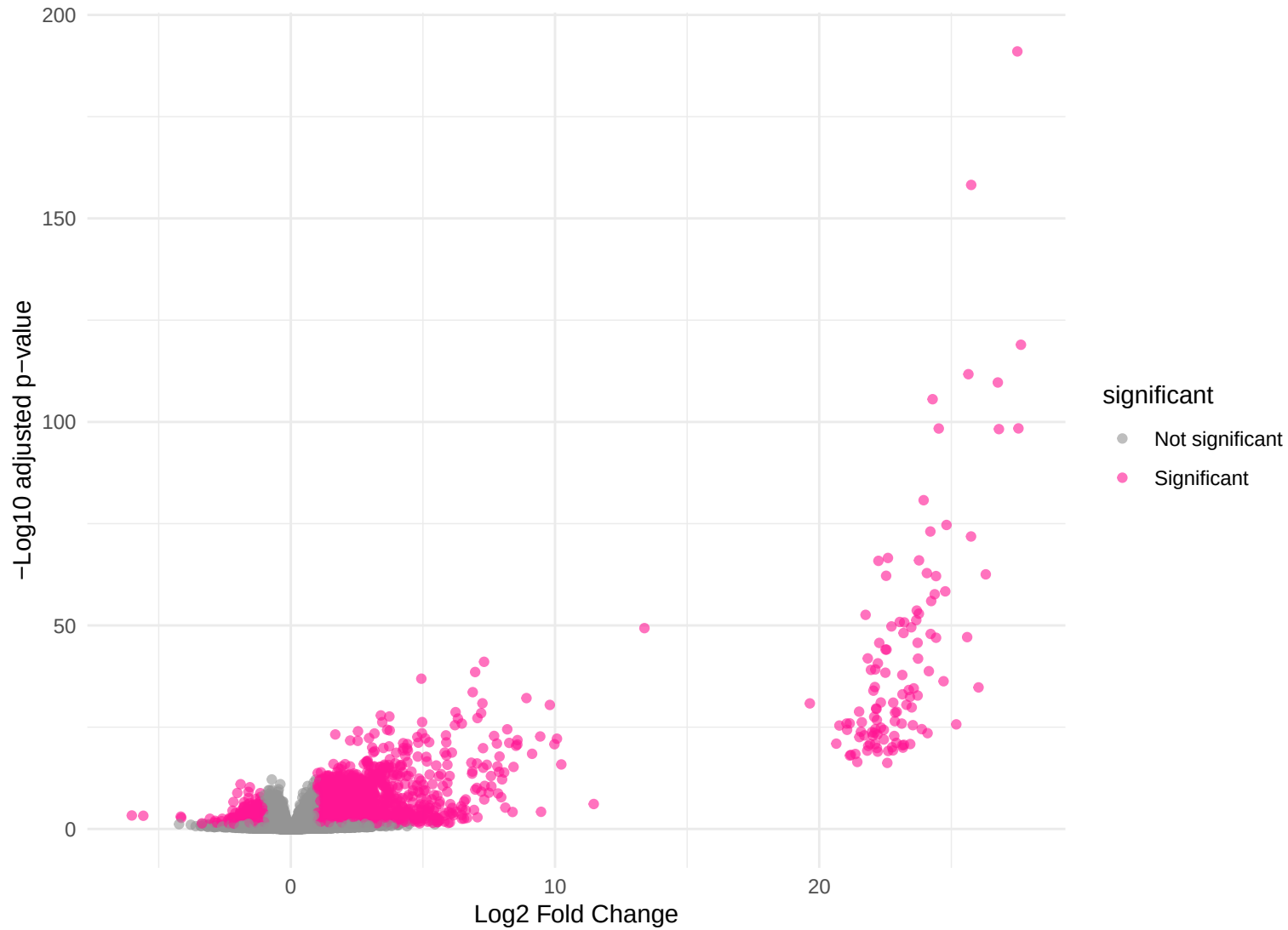
Volcano plot glioma_NE vs control
