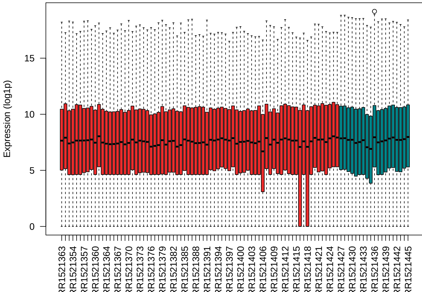
Boxplot after log1p transformation
