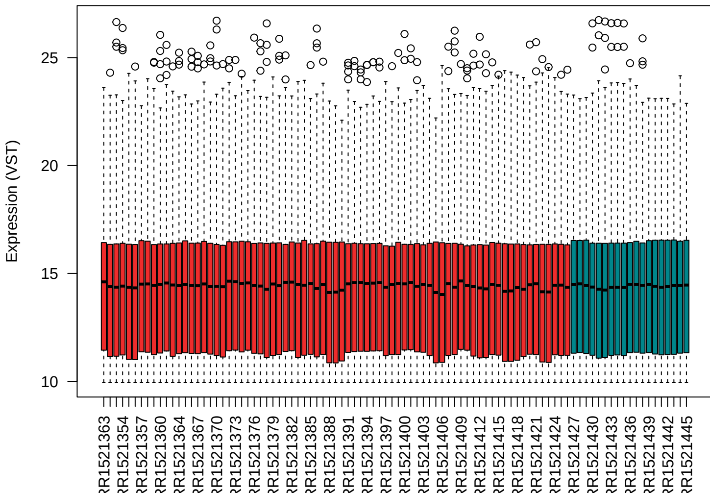
Boxplot after normalization
