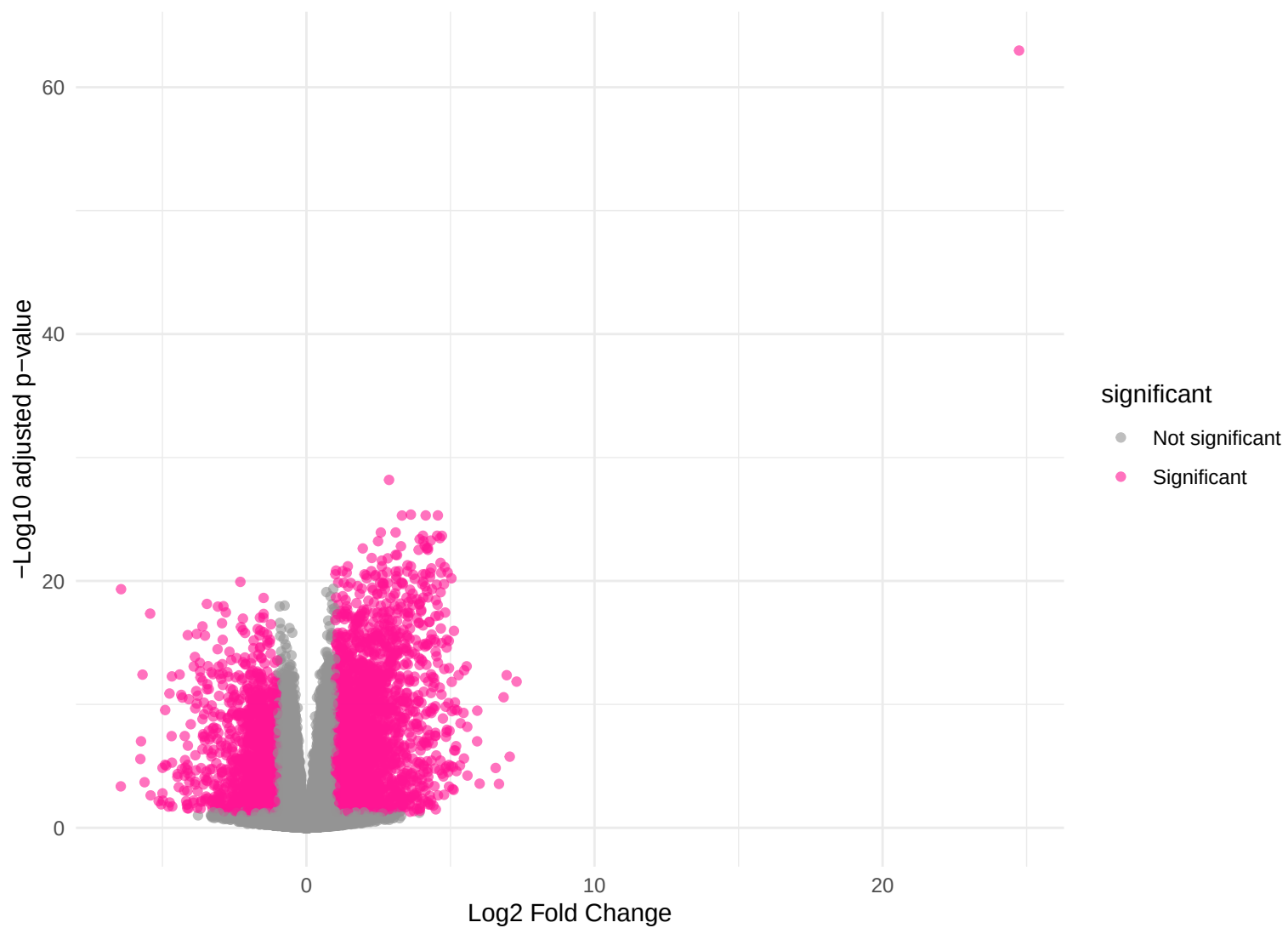
Volcano plot glioma_NE vs glioma_CE
