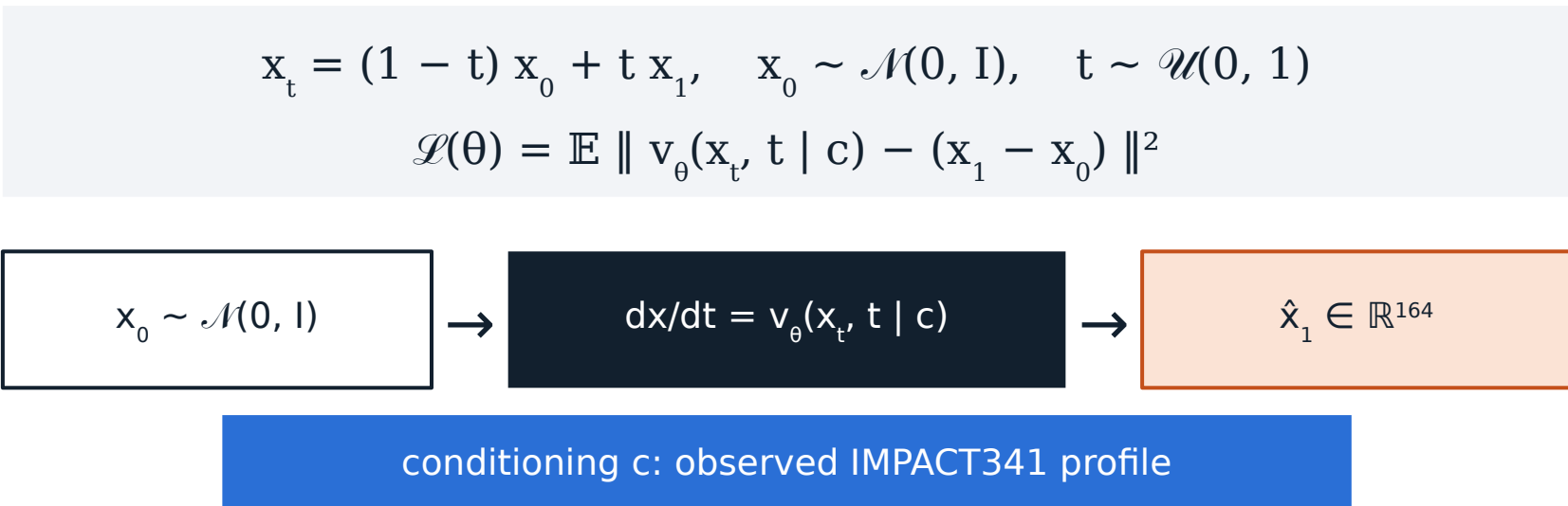
Figure 2. Sampling: the learned ODE, integrated numerically from t = 0 to 1 , transports noise to a completed 164-gene profile conditioned on the observed panel.
