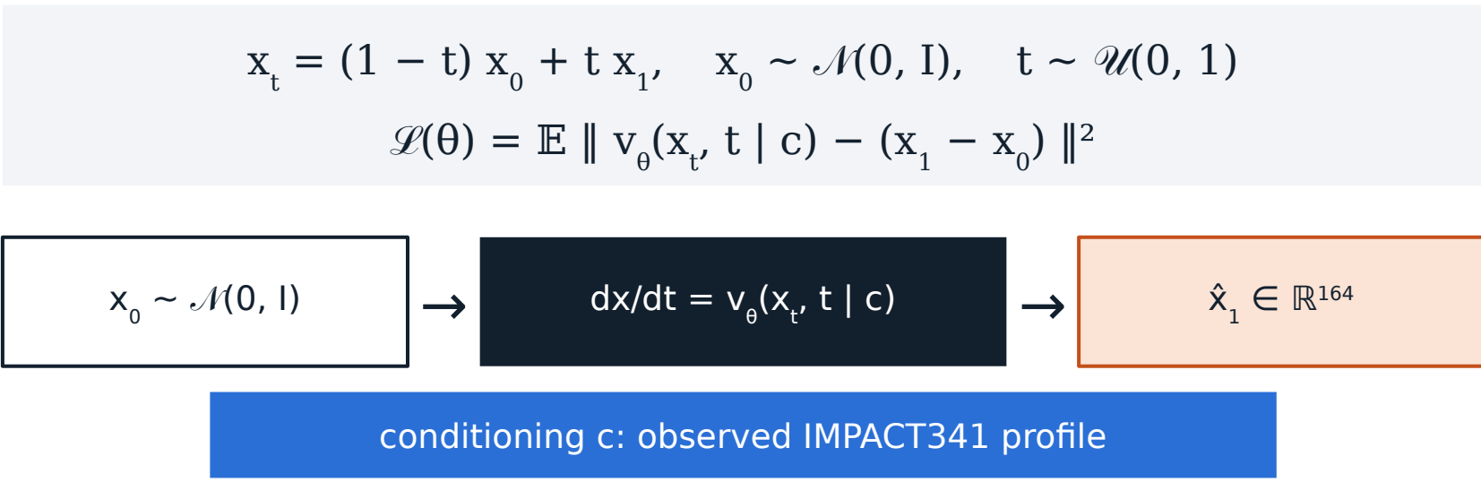
Figure 2. Sampling: the learned ODE, integrated from t = 0 to 1 ([solver, N steps]), transports noise to a completed 164-gene profile conditioned on the observed panel.
