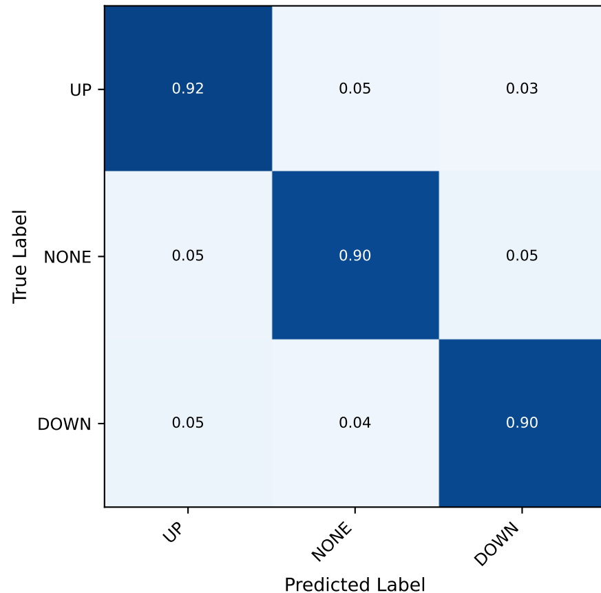
Vertical Head Confusion Matrix
