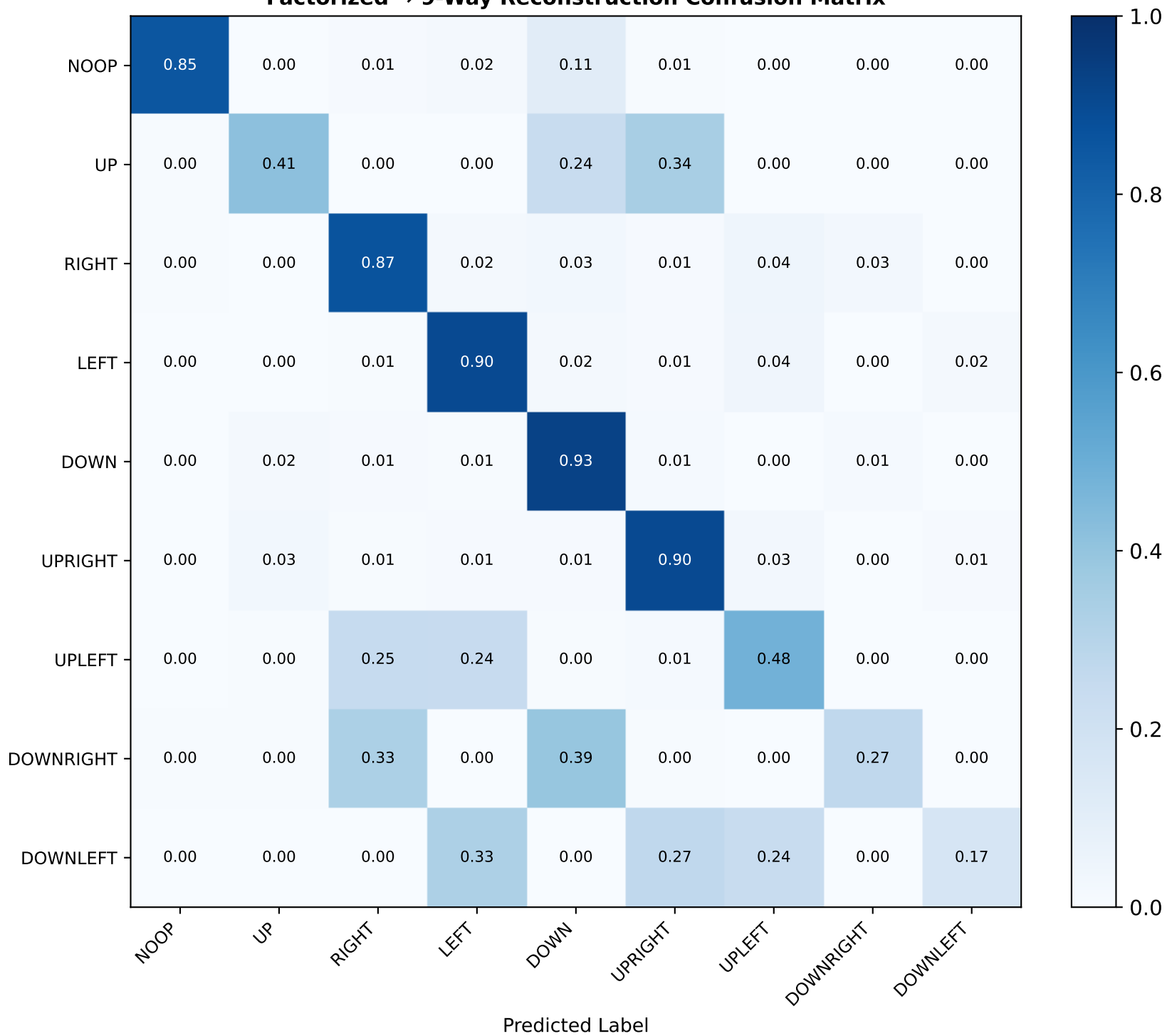
Factorized → 9-Way Reconstruction Confusion Matrix
