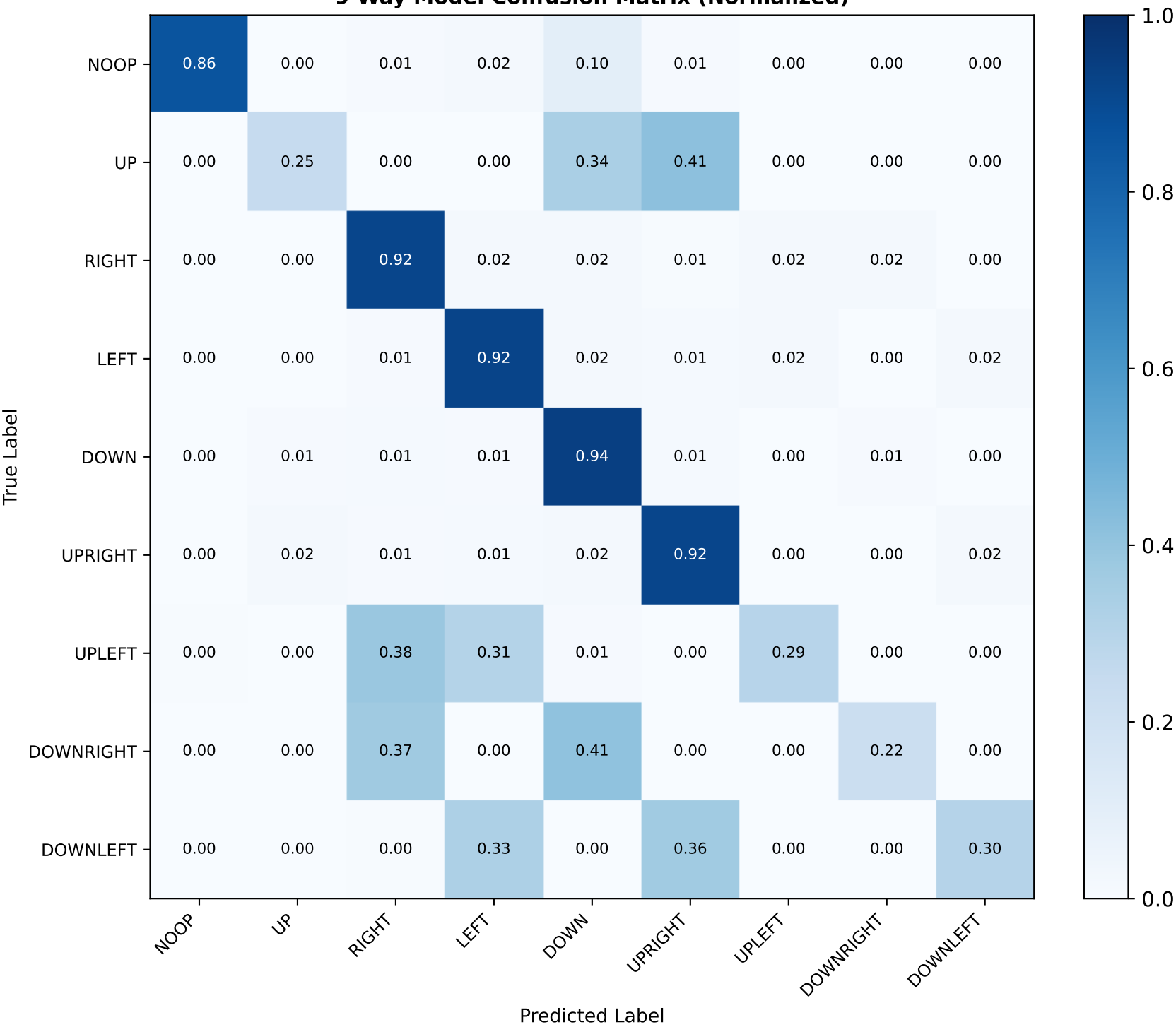
9-Way Model Confusion Matrix (Normalized)
