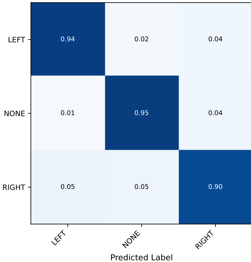
Horizontal Head Confusion Matrix
