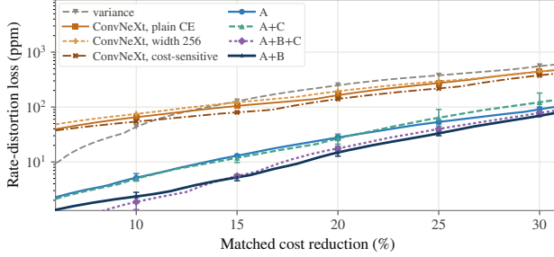
Fig. 2. Rate-distortion loss against matched cost reduction, logarithmic vertical axis. Bars give the amplitude over three seeds. The random control of Table I is omitted, as it alone spans a decade of the axis.
