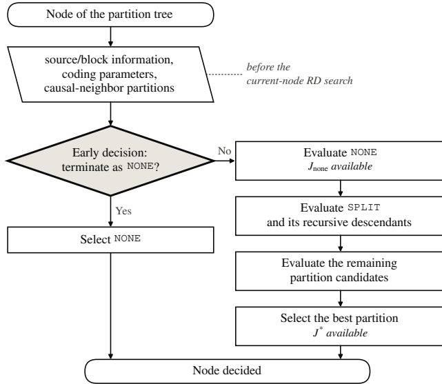
Fig. 1. AV1 intra partition-search flow highlighting the pre-search early-termination point considered in this work.
