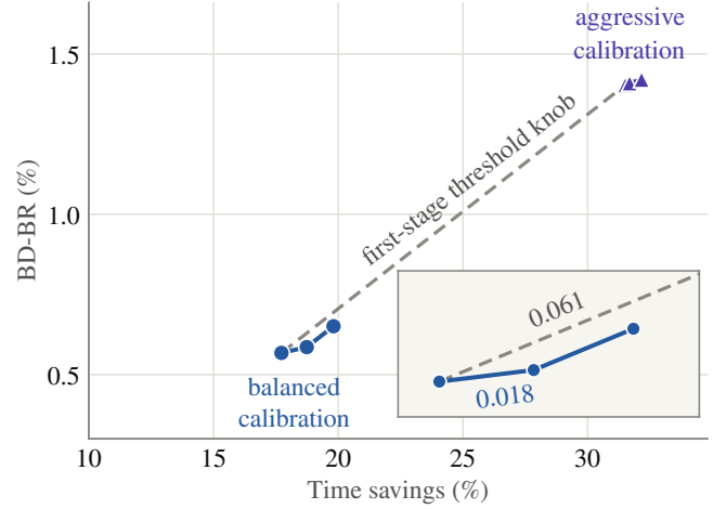
Fig. 3. Operating space of SNP-AV1 over the CTC Class A1 4K sequences. Both axes are measured against the libaom v3.10.0 anchor at cpu-used=0 , which is their origin and lies outside the plotted range. Inside each calibration the three points differ only in the strength of the second pruner, and the dashed line is the threshold knob of the first stage. The inset magnifies the balanced calibration, where the two prices, in BD-BR points per point of time savings, leave the same operating point.
