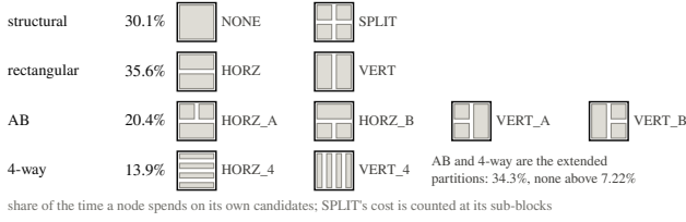
Fig. 1. The ten partition shapes evaluated at a node, grouped into the four families used in this work and annotated with the share of local search time each family consumes.
