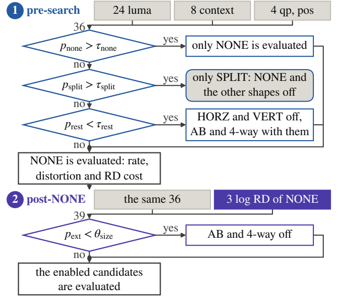
Fig. 2. Insertion points of the two pruners in the search of a node, and the cascade of conditions each of them applies.
