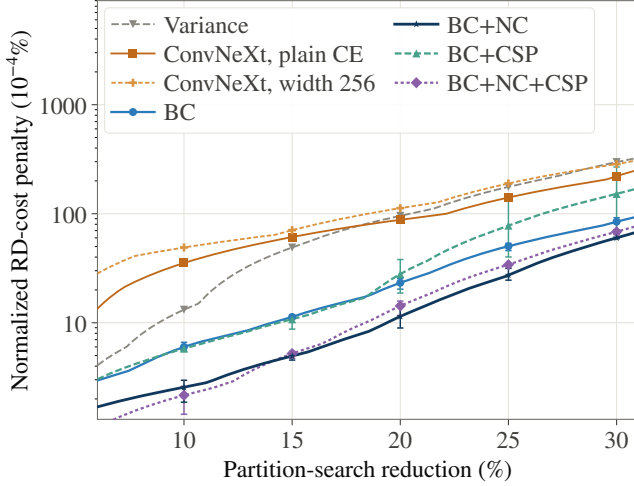
Fig. 2. Normalized RD-cost penalty as a function of partition-search reduction. Error bars show the range across three random seeds. The random control in Table 1 is omitted for readability.
