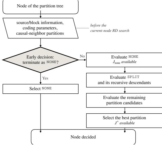
Fig. 1. AV1 intra partition-search flow highlighting the pre-search early-termination point considered in this work.
