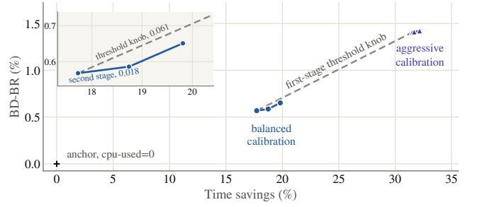
Fig. 3. Operating space of SNP-AV1 over the CTC Class A1 4K sequences, against the libaom v3.10.0 anchor at cpu-used=0 . Inside each calibration the three points differ only in the strength of the second pruner; the dashed line is the threshold knob of the first stage, and the inset resolves the balanced calibration, where the two prices leave the same operating point.
