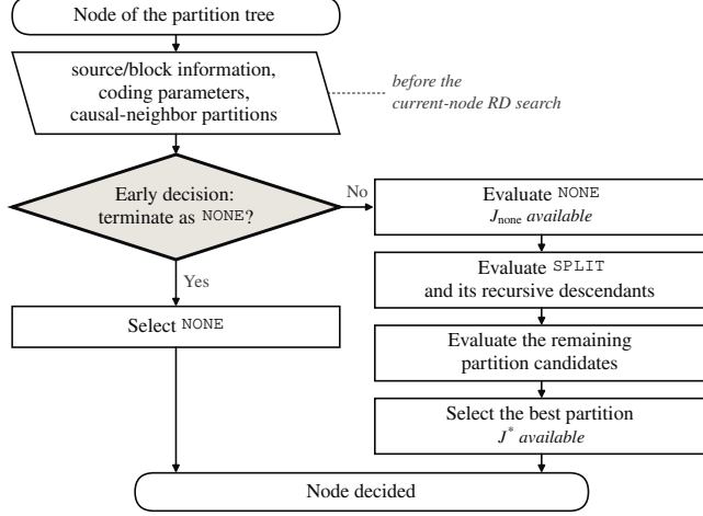
Fig. 1. AV1 intra partition-search flow highlighting the pre-search early-termination point considered in this work.
