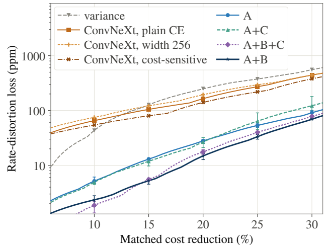
Fig. 2. Rate-distortion loss against matched cost reduction, logarithmic vertical axis. Bars give the amplitude over three seeds. The random control of Table 1 is omitted, as it alone spans a decade of the axis.
