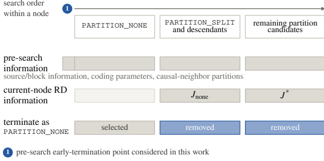
Fig. 1. AV1 intra partition-search flow highlighting the pre-search early-termination point considered in this work.
