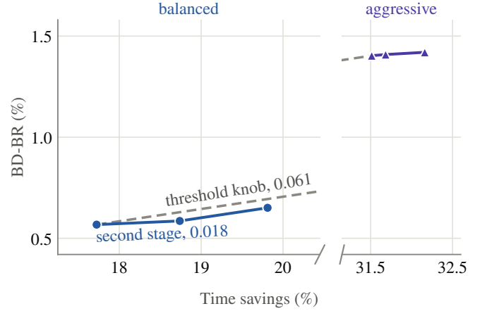
Fig. 3. Operating space of SNP-AV1 over the CTC Class A1 4K sequences, measured against the libaom v3.10.0 anchor at cpu-used=0 , which is the origin of both axes. The time axis is broken into two windows of the same scale, the balanced calibration on the left and the aggressive one on the right, over a common BD-BR axis. Inside each window the three points differ only in the strength of the second pruner; the dashed line is the threshold knob of the first stage, and the two annotated slopes are the prices of the two levers, in BD-BR points per point of time savings.
